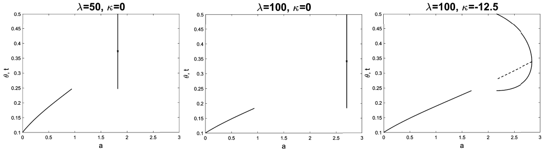
FIGURE 3.—Equilibrium actions for different values of \lambda and \kappa . Higher \lambda corresponds to larger returns to signaling. The case of \kappa = -12.5 corresponds to a type distribution with thinner right tail than the uniform distribution. The dotted line shows the locus of (S(\theta), T(\theta)) in the (a, t) -space above the gap. The solid line plots a = S(\theta) against \theta .
