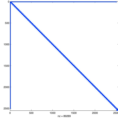
(b) Sparsity Pattern of the Hessian
