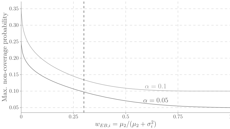
FIGURE 4.—Maximal non-coverage probability of parametric EB CI, \alpha \in \{0.05, 0.10\} . The vertical line marks the “rule of thumb” value w_{EB,i} = 0.3 , above which the maximal coverage distortion is less than 5 percentage points for these two values of \alpha .
