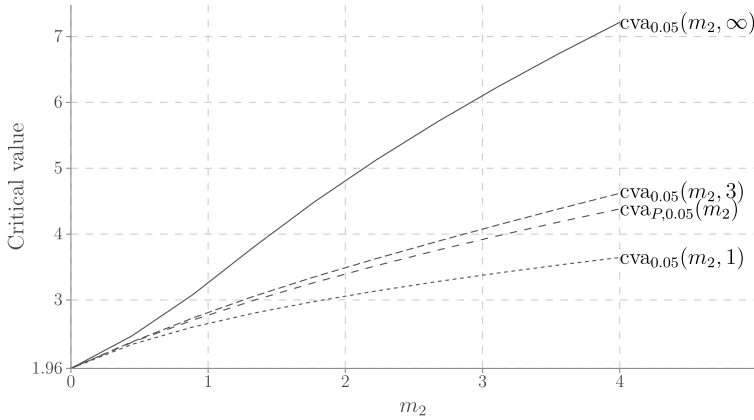
FIGURE 1.—Function cva_{\alpha}(m_2, \kappa) for \alpha = 0.05 and selected values of \kappa . The function cva_{\alpha}(m_2) , defined in Section 2, that only imposes a constraint on the second moment, corresponds to cva_{\alpha}(m_2, \infty) . The function cva_{p,\alpha}(m_2) = z_{1-\alpha/2}\sqrt{1+m_2} corresponds to the critical value under the assumption that \theta_i is normally distributed.
