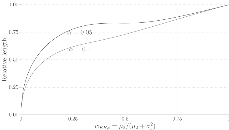
FIGURE 3.—Efficiency of robust EBCI \hat{\theta}_i \pm \text{cva}_\alpha(\sigma_i^2/\mu_2, \kappa = \infty) \cdot \sigma \mu_2 / (\mu_2 + \sigma_i^2) relative to the unshrunk CI Y_i \pm z_{1-\alpha/2} \sigma_i . The figure plots the ratio of the length of the robust EBCI relative to the unshrunk CI as a function of the shrinkage factor w_{\text{EB},i} = \mu_2/(\mu_2 + \sigma_i^2) .
