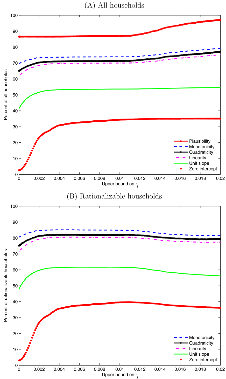
FIGURE S3. Increasing the upper bound on r_i .
