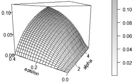
(a) Comparison of average distances between optimal risk-averse and risk-neutral decisions, |d_1^{\text{RA}} - d_2^{\text{RA}}| - |d_1^{\text{RN}} - d_2^{\text{RN}}| for \gamma = \frac{1}{4} . Each point corresponds to the average over (\nu_1, \nu_2) \in [-0.6, 0.6]^2 with a grid of size 0.05.
