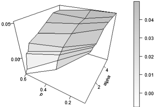
(b) Comparison of average distances between optimal maxmin and risk/ambiguity-neutral decisions, |d_1^{AA} - d_2^{AA}| - |d_1^{RN} - d_2^{RN}| for \gamma = \frac{3}{4} , different degrees of risk aversion \alpha , and different distribution parameters p . Each point corresponds to the average over (\nu_1, \nu_2) \in [-0.6, 0.6]^2 with a grid of size 0.05. The grid size for the decisions is 0.05, and the value of \epsilon = 0.4 .
