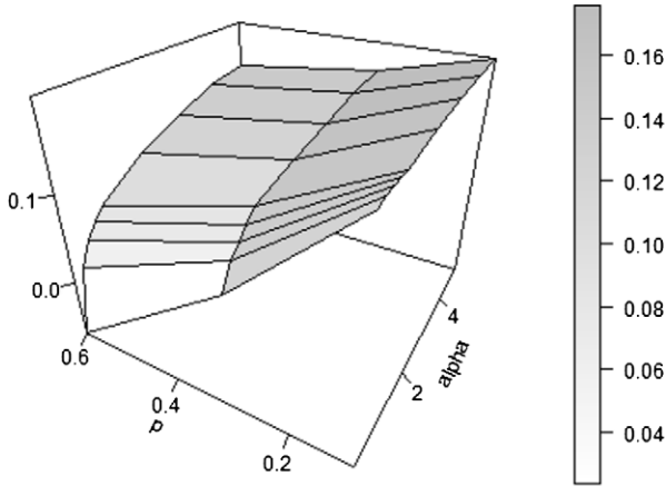
(a) Comparison of average distances between optimal maxmin and risk/ambiguity-neutral decisions, |d_1^{AA} - d_2^{AA}| - |d_1^{RN} - d_2^{RN}| for \gamma = \frac{1}{4} , different degrees of risk aversion \alpha , and different distribution parameters p . Each point corresponds to the average over (\nu_1, \nu_2) \in [-0.6, 0.6]^2 with a grid of size 0.05. The grid size for the decisions is 0.05, and the value of \epsilon = 0.4 .
