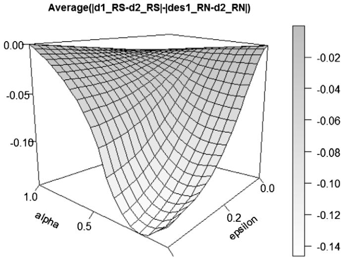
(a) Comparison of average distances between optimal risk-seeking and risk-neutral decisions, |d_1^{\text{RS}} - d_2^{\text{RS}}| - |d_1^{\text{RN}} - d_2^{\text{RN}}| for \gamma = \frac{1}{4} . Each point corresponds to the average over (\nu_1, \nu_2) \in [-0.6, 0.6]^2 with a grid of size 0.05. The grid size for \alpha is 0.05.
