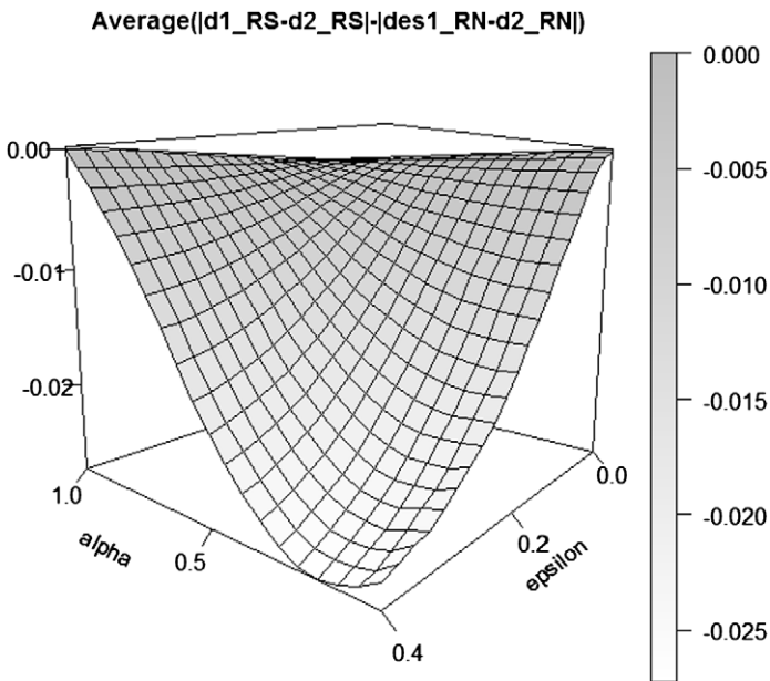
(b) Comparison of average distances between optimal risk-seeking and risk-neutral decisions, |d_1^{\text{RS}} - d_2^{\text{RS}}| - |d_1^{\text{RN}} - d_2^{\text{RN}}| for \gamma = \frac{3}{4} . Each point corresponds to the average over (\nu_1, \nu_2) \in [-0.6, 0.6]^2 with a grid of size 0.05. The grid size for \alpha is 0.05.
