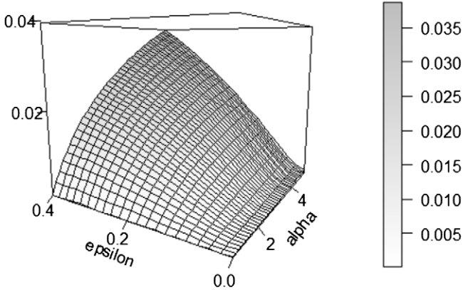
(b) Comparison of average distances between optimal risk-averse and risk-neutral decisions, |d_1^{\text{RA}} - d_2^{\text{RA}}| - |d_1^{\text{RN}} - d_2^{\text{RN}}| for \gamma = \frac{3}{4} . Each point corresponds to the average over (\nu_1, \nu_2) \in [-0.6, 0.6]^2 with a grid of size 0.05.
