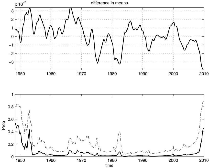
FIGURE 8. The one-noise system. Difference in means (top panel) and Bayesian model probability \tilde{\iota}_t (solid line) and worst-case model probability \tilde{\iota}_t^* (dashed line) (bottom panel).
