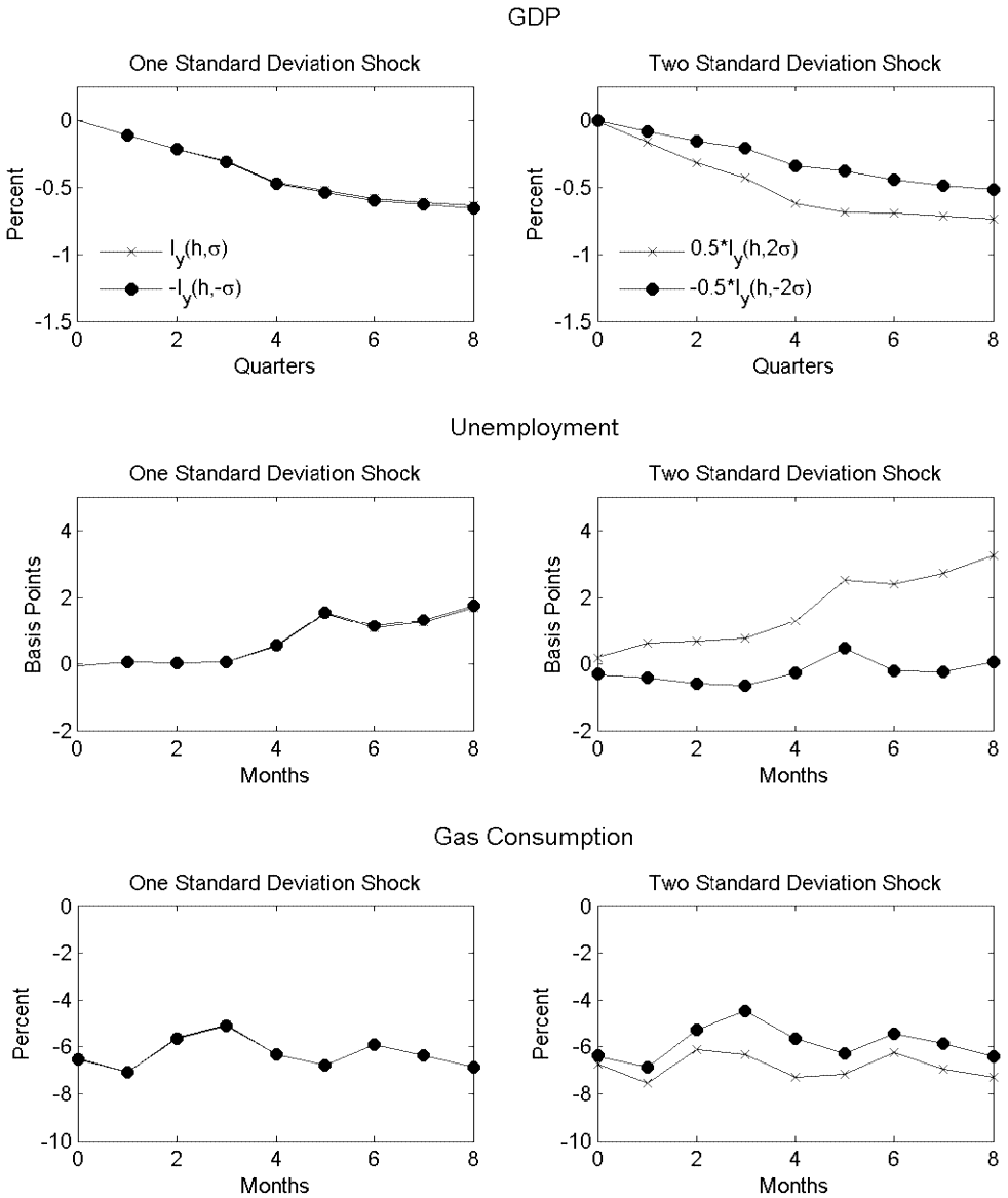
FIGURE 7. Empirical responses to 1 and 2 standard deviation positive and negative energy price shocks in baseline model with 6 lags: 3-year net increase. The responses to negative shocks are shown as mirror images to facilitate the comparison. Some of the responses in the left panel are nearly invisible because the responses are almost perfectly symmetric.
