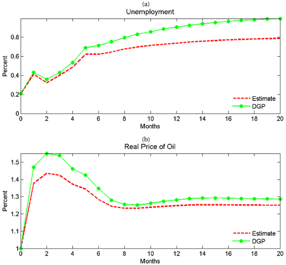
FIGURE 4. Inconsistency of the estimated effect of unanticipated oil price increases for the asymmetric structural model DGP: Fitting the censored VAR model. Simulations based on model (11) estimated on U.S. data. T = 1,000,000 .
