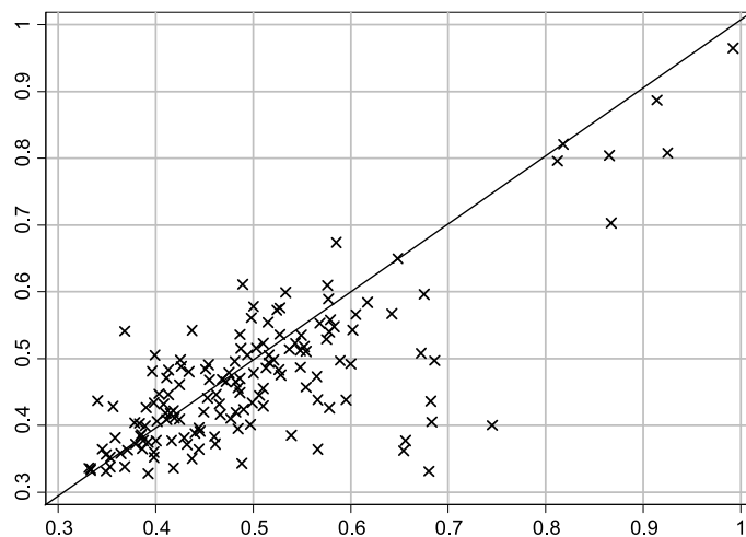
FIGURE 5. Scatterplot of the average fraction of tokens allocated to the cheapest security by subject. Vertical axis : The average fraction of tokens allocated to the cheapest security (the security with the lowest price) when it pays off in an ambiguous state. Horizontal axis : The average fraction of tokens allocated to the cheapest when it pays off in the unambiguous state.
