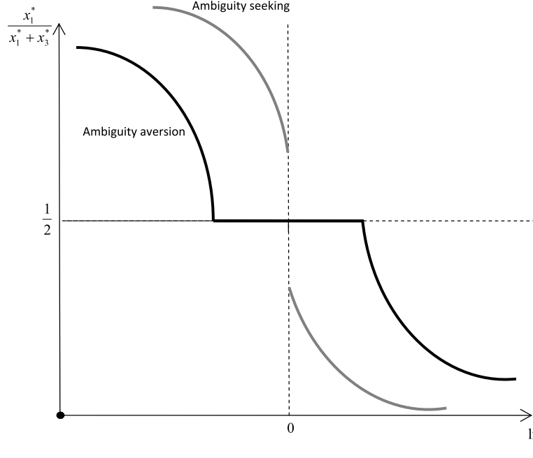
FIGURE 6. An illustration of the relationships between log-price ratio and the optimal token share of the securities that pay off in the ambiguous states in the kinked specification (equation (1)).
