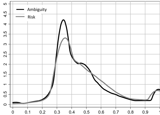
FIGURE 3. The distribution of the fraction of tokens allocated to the cheapest security (kernel density estimates). Kernel density estimates of the token share of the cheapest security (the security with the lowest price). Black : Portfolios where the cheapest security pays off in one of the ambiguous states, 1 or 3. Gray : Portfolios where the cheapest security pays off in the unambiguous state.
