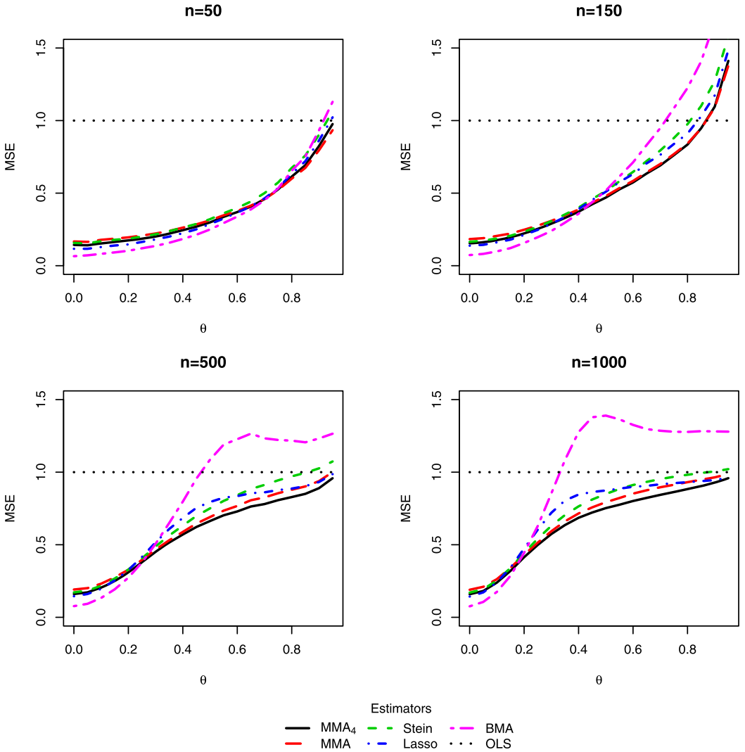
FIGURE 5. Autoregression.
