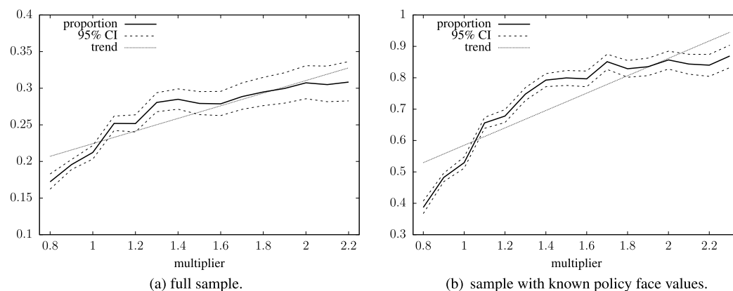
FIGURE 4. Proportion of policyholders that settled their policy as a function of the mortality multiplier (solid curve), with pointwise 95% confidence intervals (dashed curves); earliest observation date. Left panel: Proportion calculated based on the full sample. Right panel: Proportion calculated based only on policies with known face values in the remaining sample.
