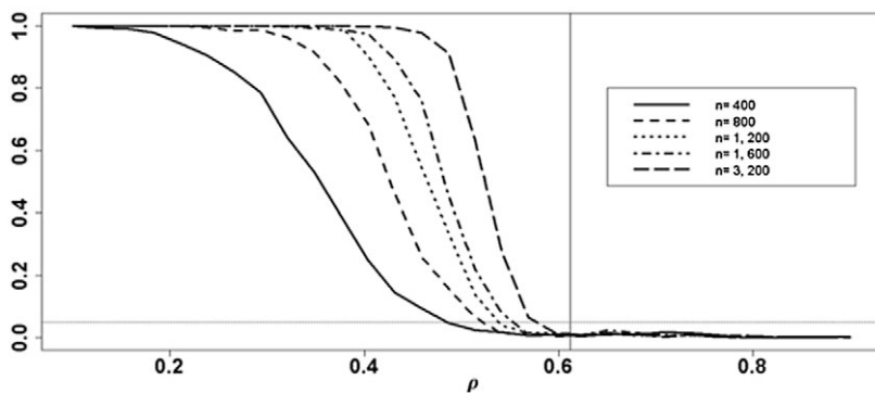
FIGURE 1. Power curves. Notes: The vertical line at \rho \simeq 0.616 corresponds to the theoretical limit for the rejection of the null hypothesis using our test. The dotted horizontal line corresponds to the 5% level.
