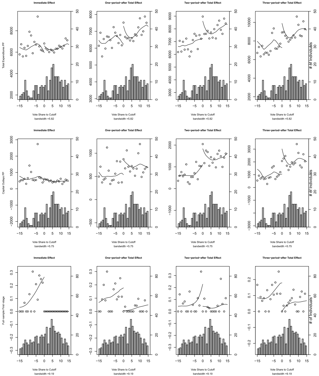
FIGURE 1. Average total effects and histograms. Note: The data set is from Cellini, Ferreira, and Rothstein (2010). The kernel bandwidth of each row is set to the same value, which is the average of CCT bandwidths among all four RD regressions of the row. The data sample of the first two rows is a subset of that of the last row, because of missing values in the expense outcomes.
